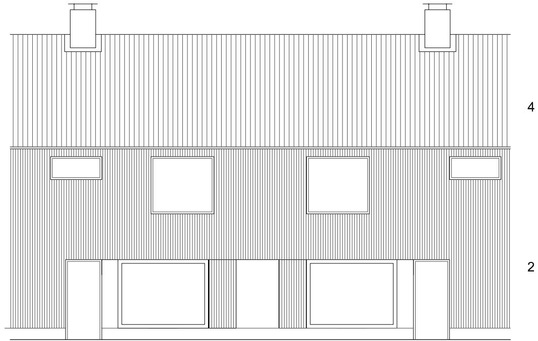
front elevation
