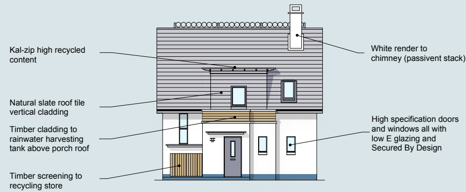
FRONT ELEVATION 1:100
