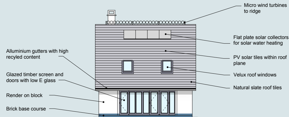
REAR ELEVATION 1:100
