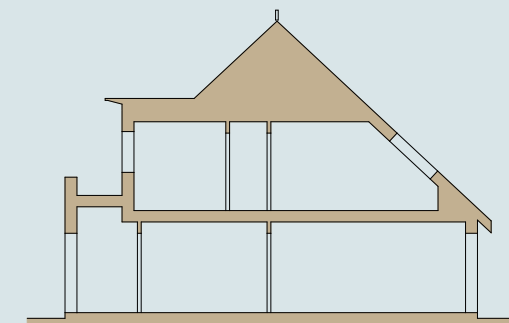
SECTION 1:100
