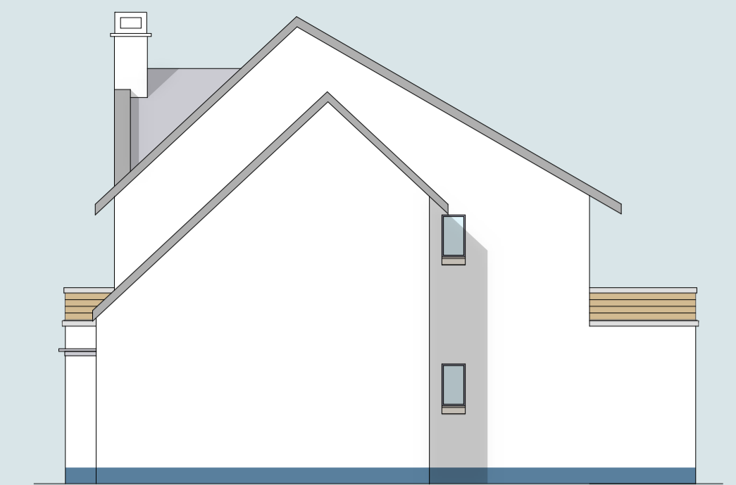
SIDE ELEVATION 1:100
